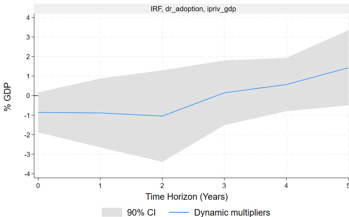
Figure 5: Impulse Response Function of Private Investment to Debt Rule Adoption
